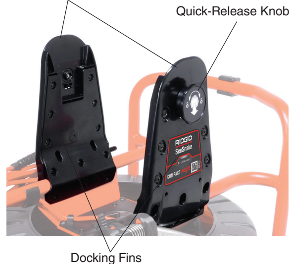
Joint Sockets
