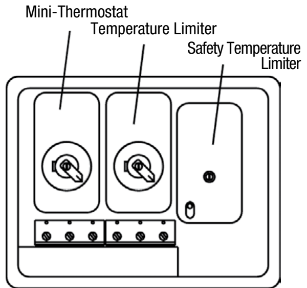
Triple Thermostat Inside View
