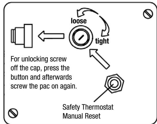
Triple Thermostat Outside View
